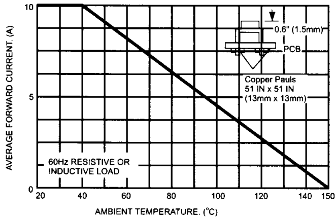
FIG.1- MAXIMUM DERATING CURVE FOR OUTPUT RECTIFIED CURRENT
