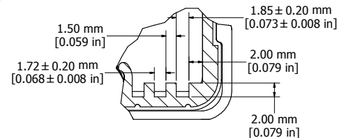
DETAIL L
