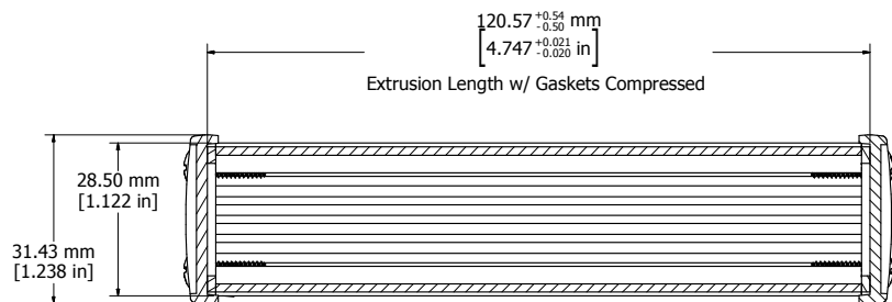
SECTION Y-Y
