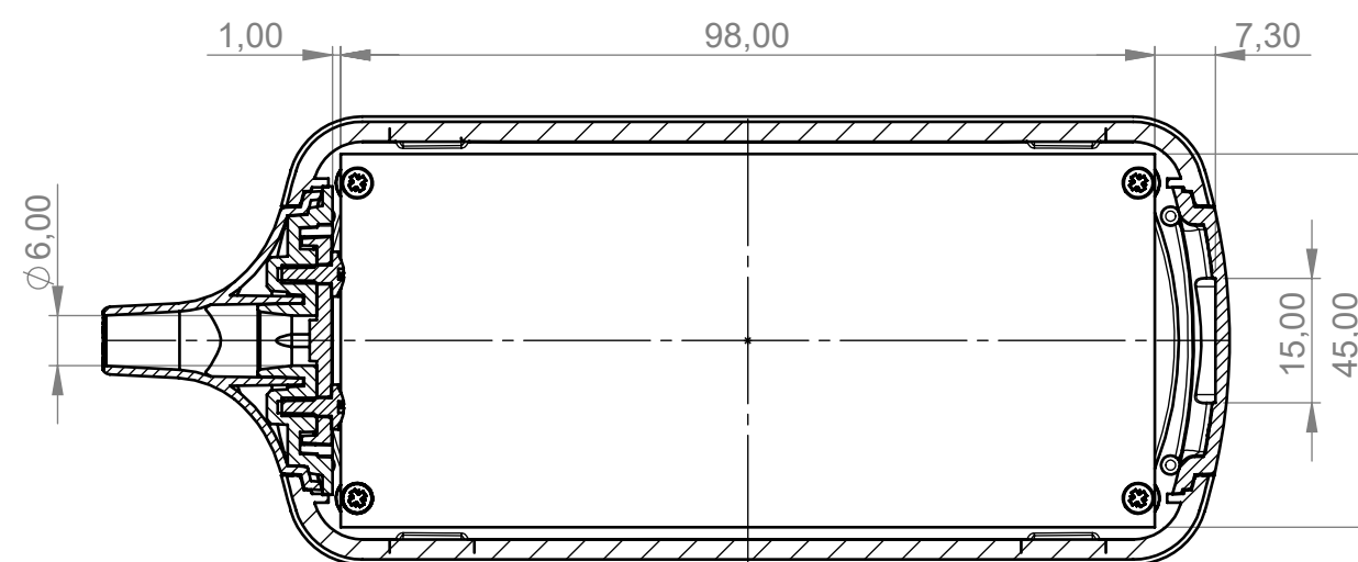
C-C flattened shell with mounted PCB -inside view-
