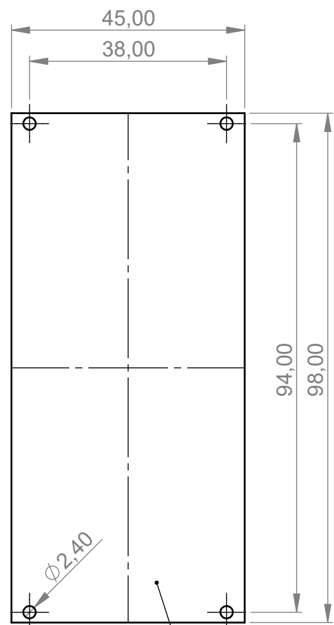
example PCB
