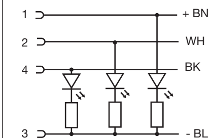
4-wire PNP angled version
