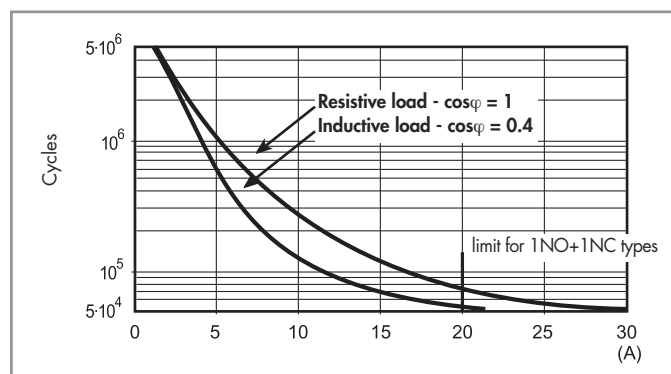
F 65 - Electrical life (AC) v contact current
