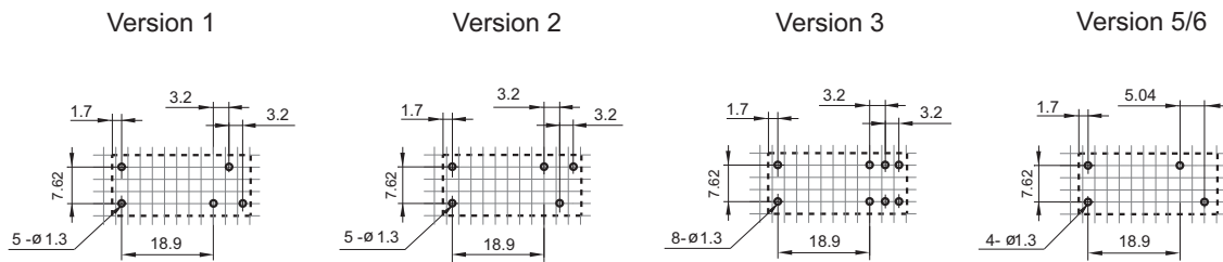
PCB Layout (Bottom view)
