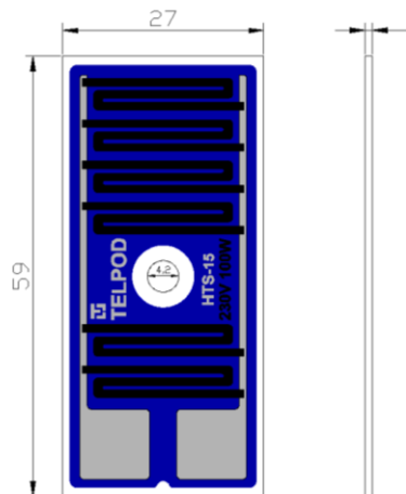
Fig. 1. Preview with dimensions [mm]
