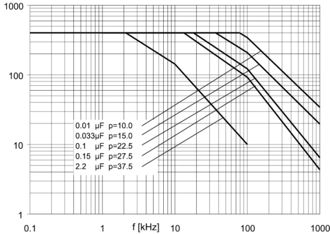
630 Vdc / 400 Vac
