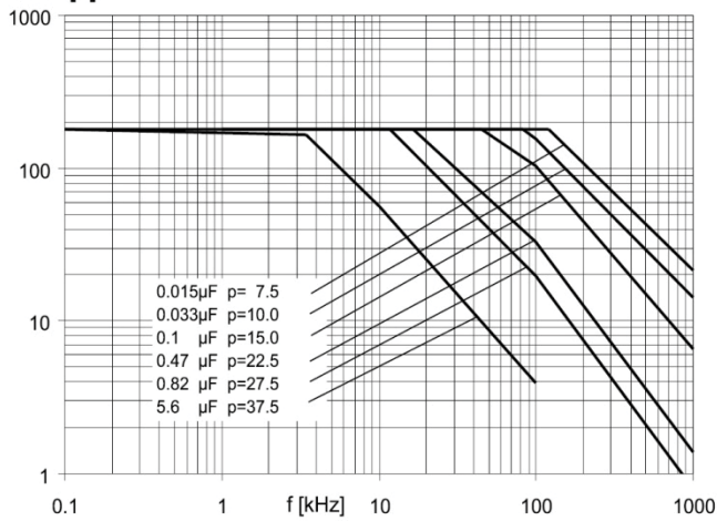
630 Vdc / 400 Vac
