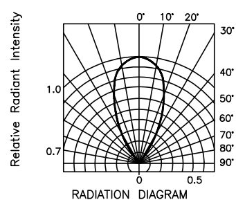
RADIATION DIAGRAM
