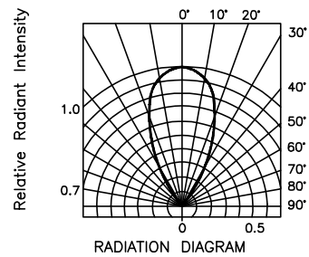
RADIATION DIAGRAM
