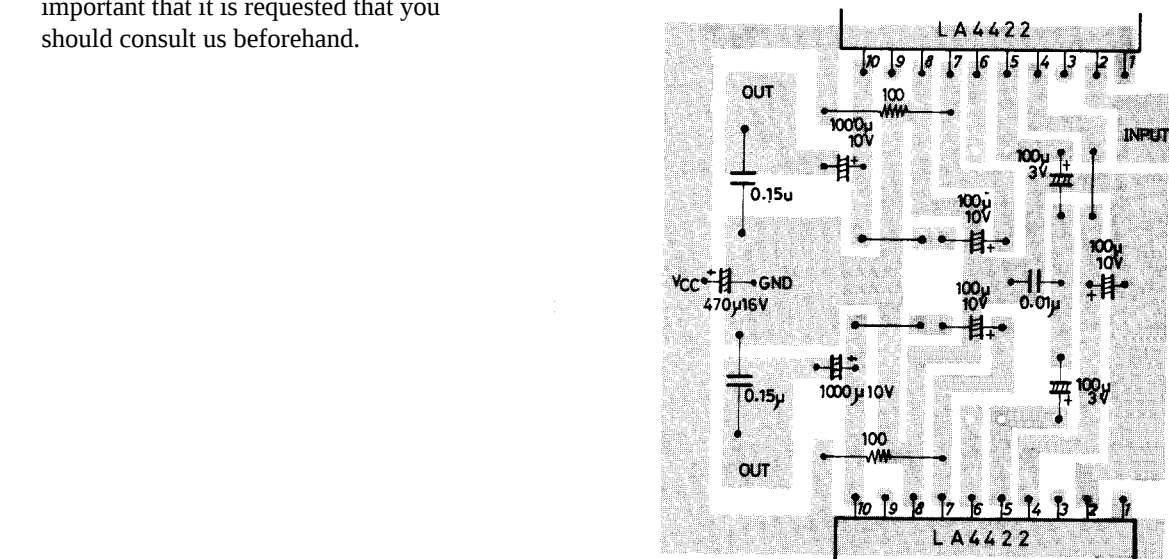
Sample Printed Circuit Pattern (45 x 43mm 3 , Cu-foiled side)
