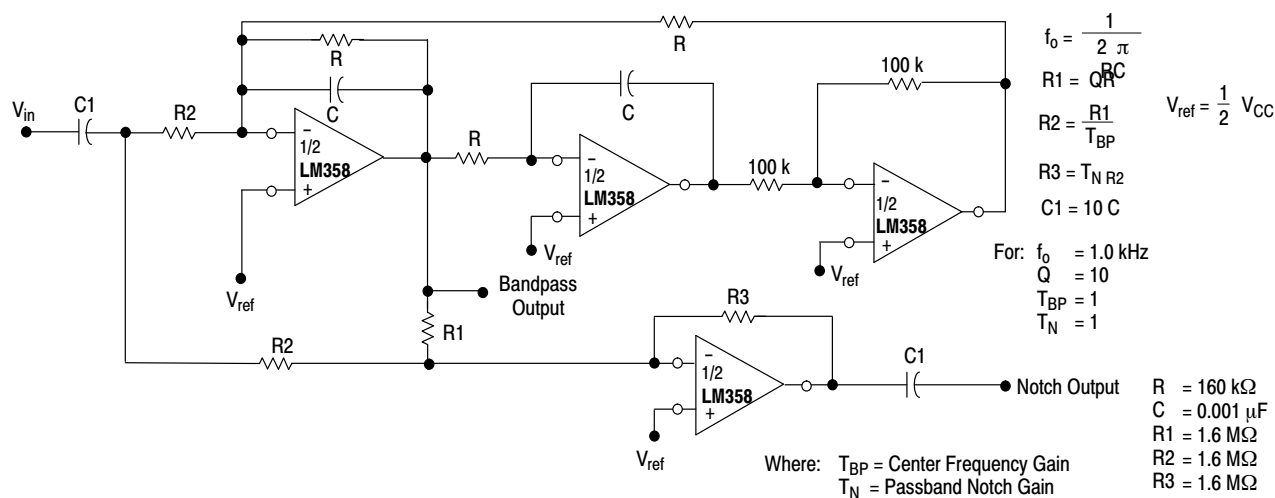
Figure 14. Bi-Quad Filter
