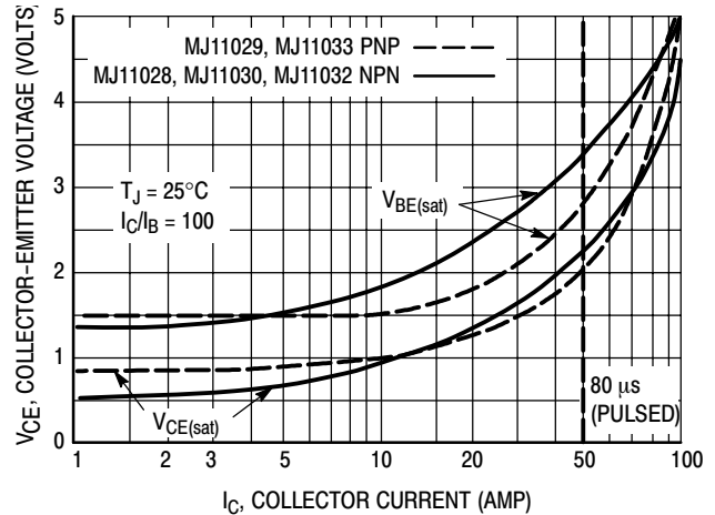
Figure 4. "On" Voltage
