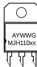
SOT-93 (TO-218) CASE 340D STYLE 1
