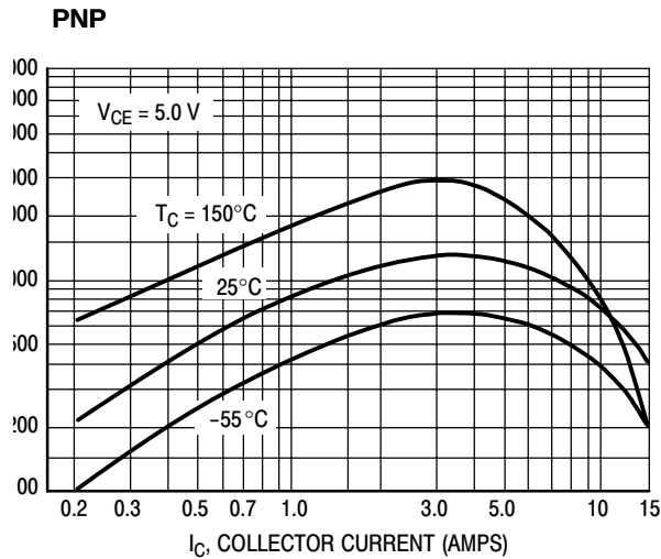
Figure 6. DC Current Gain
