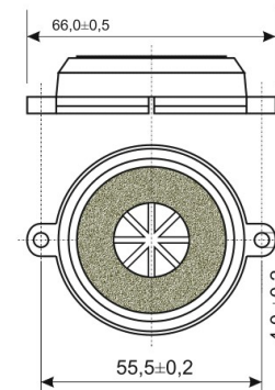
HOUSING 3
