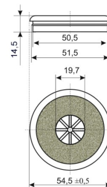
HOUSING 2
