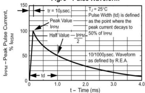
Fig. 3 – Pulse Waveform
