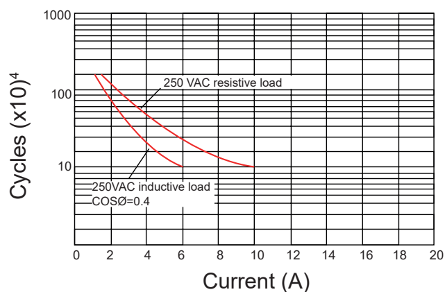
Electrical durability curve
