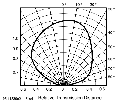
Fig. 13 - Vertical Directivity
